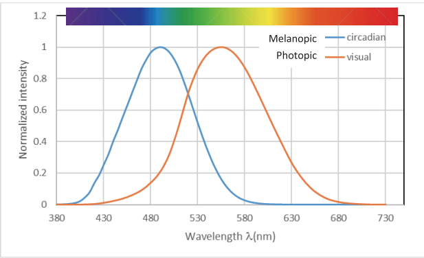
Picture1:The response curves of Photopic and Melanopic in humans; Melanopic Ratio of Standard LED Light Sources
