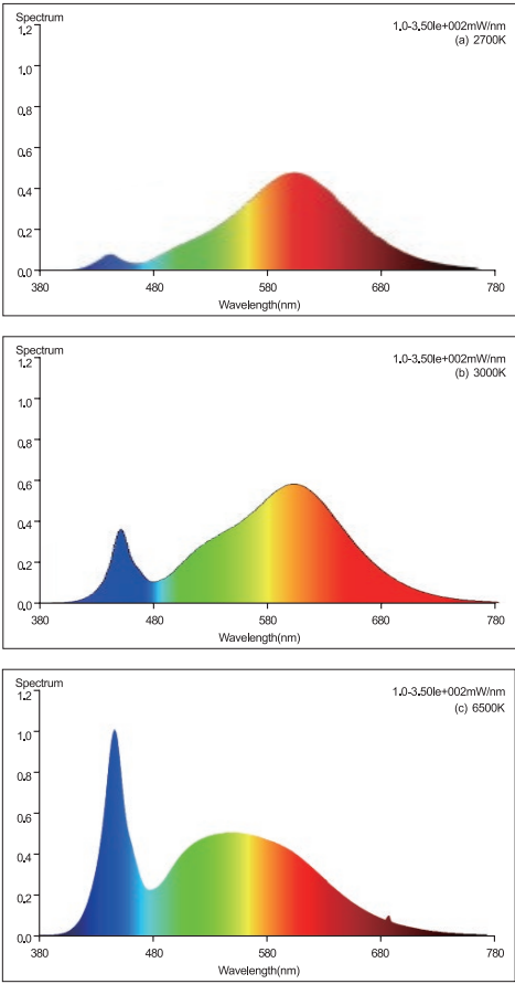
Picture3:The LED light source with three different CCTs can customize the spectrum and achieve the required MR Ratio;
